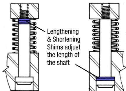
Lengthening Shims
